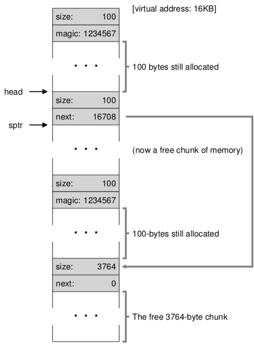
Figure 17.6: Free Space With Two Chunks Allocated
