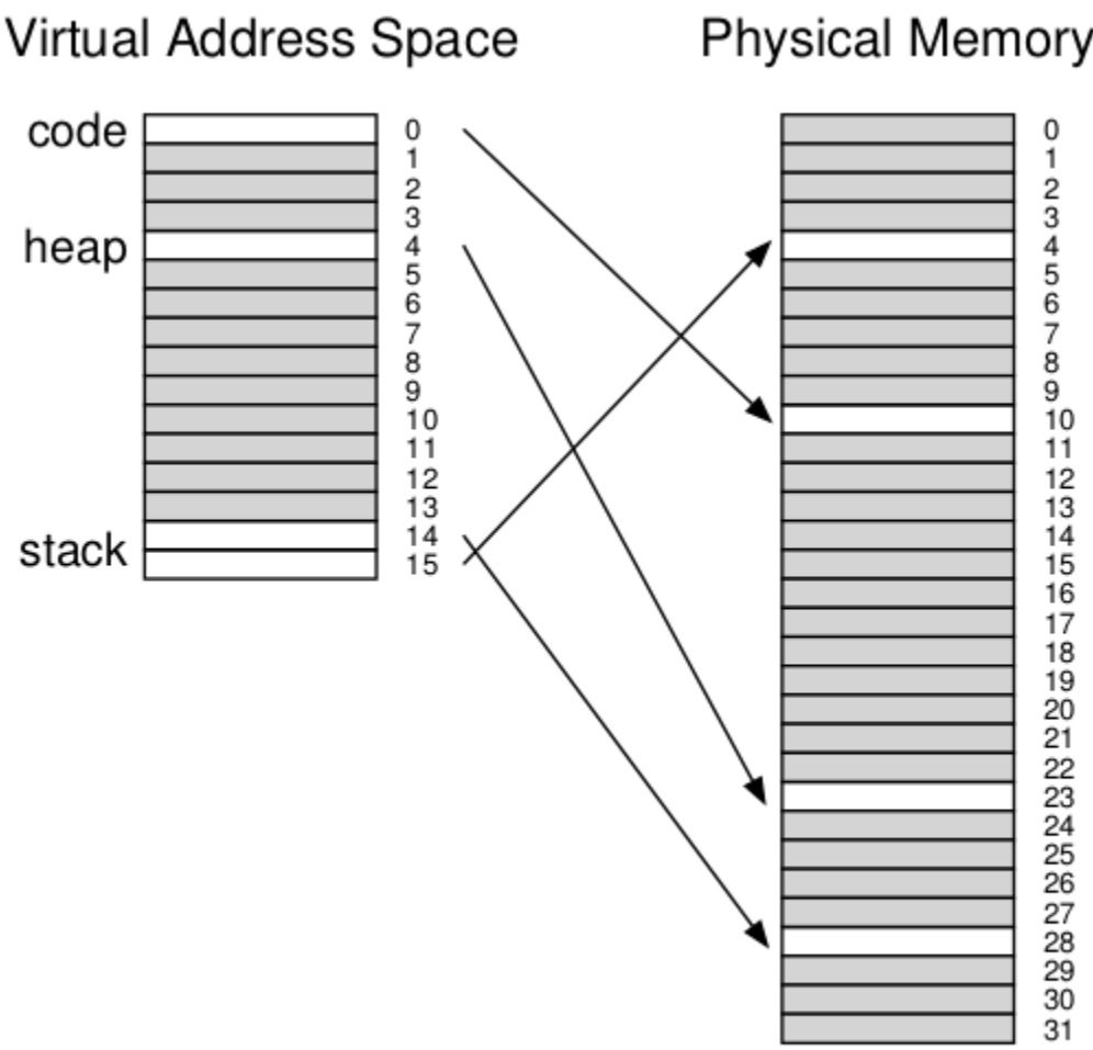
Figure 20.1: A 16KB Address Space With 1KB Pages
