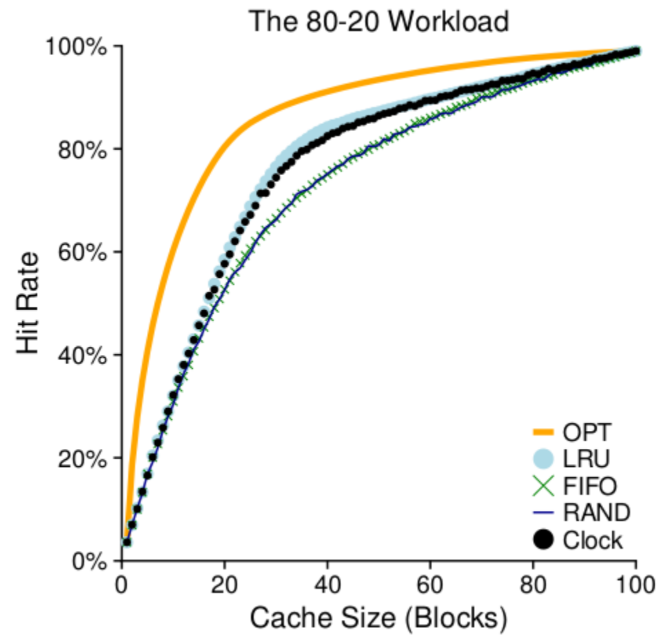
Figure 22.9: The 80-20 Workload With Clock
